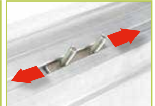
EASY SLIDE FIXING FOR RAFTERS
